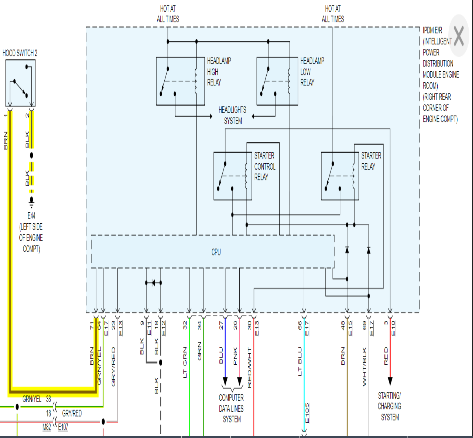
Theft - Forced Entry Circuit
