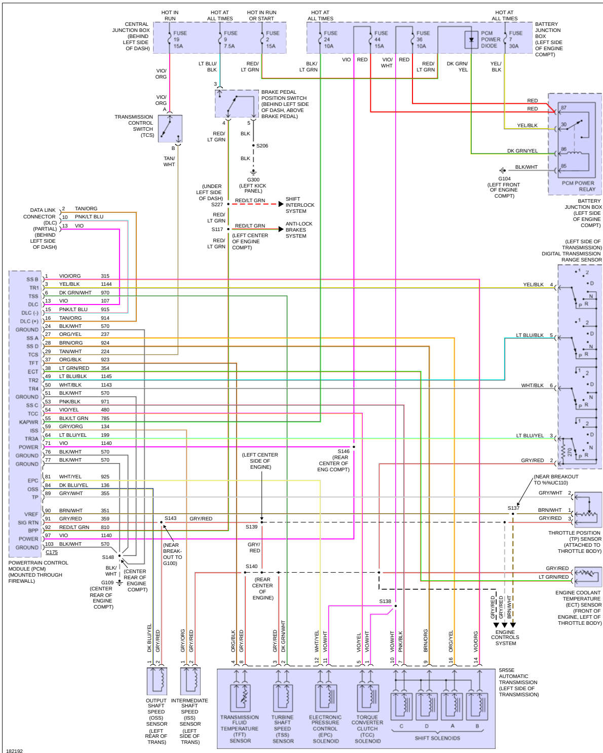
Fig 2: A/T Circuit
