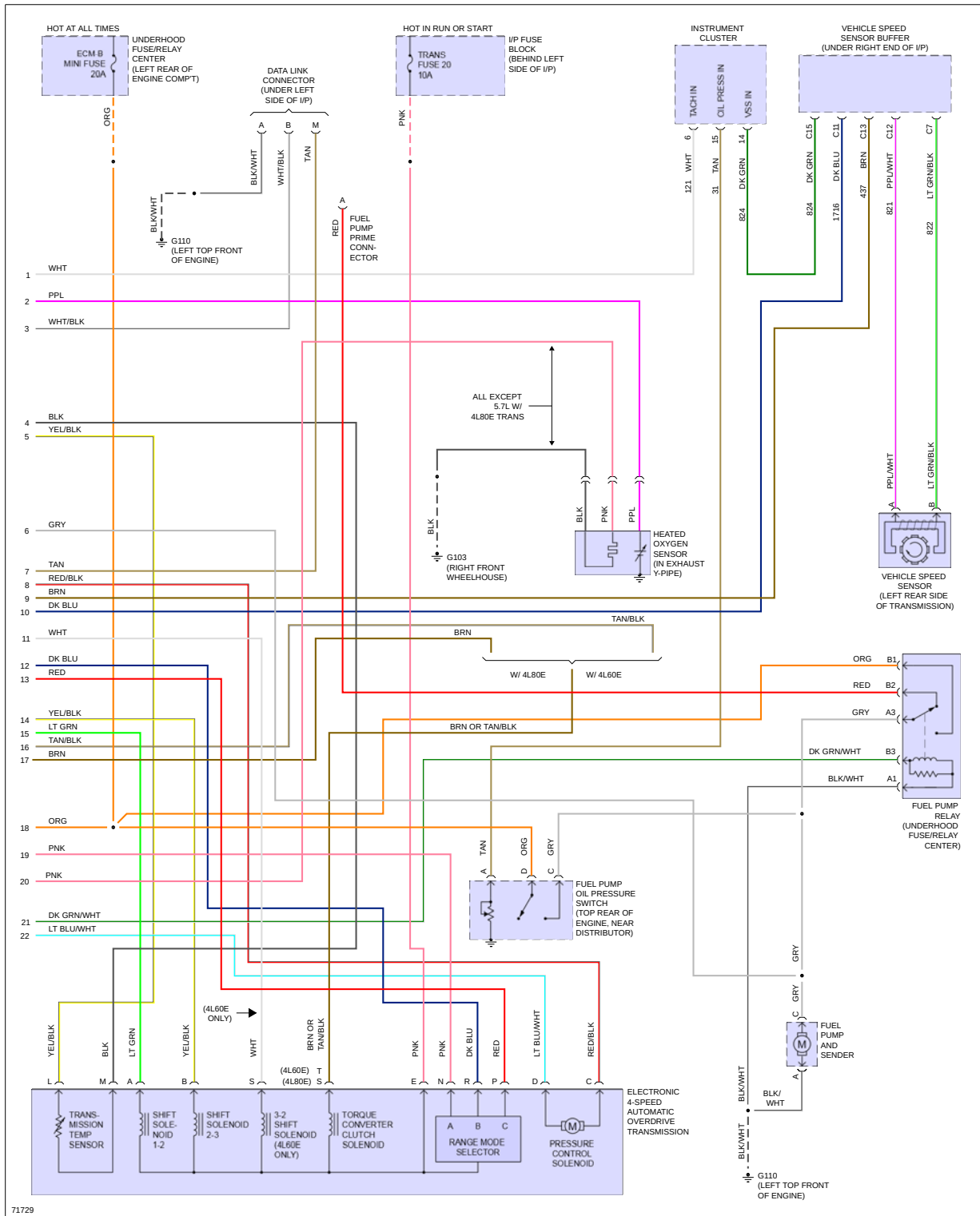
Fig 3: 5.7L (VIN K), Engine Performance Circuits, A/T (3 of 3)
