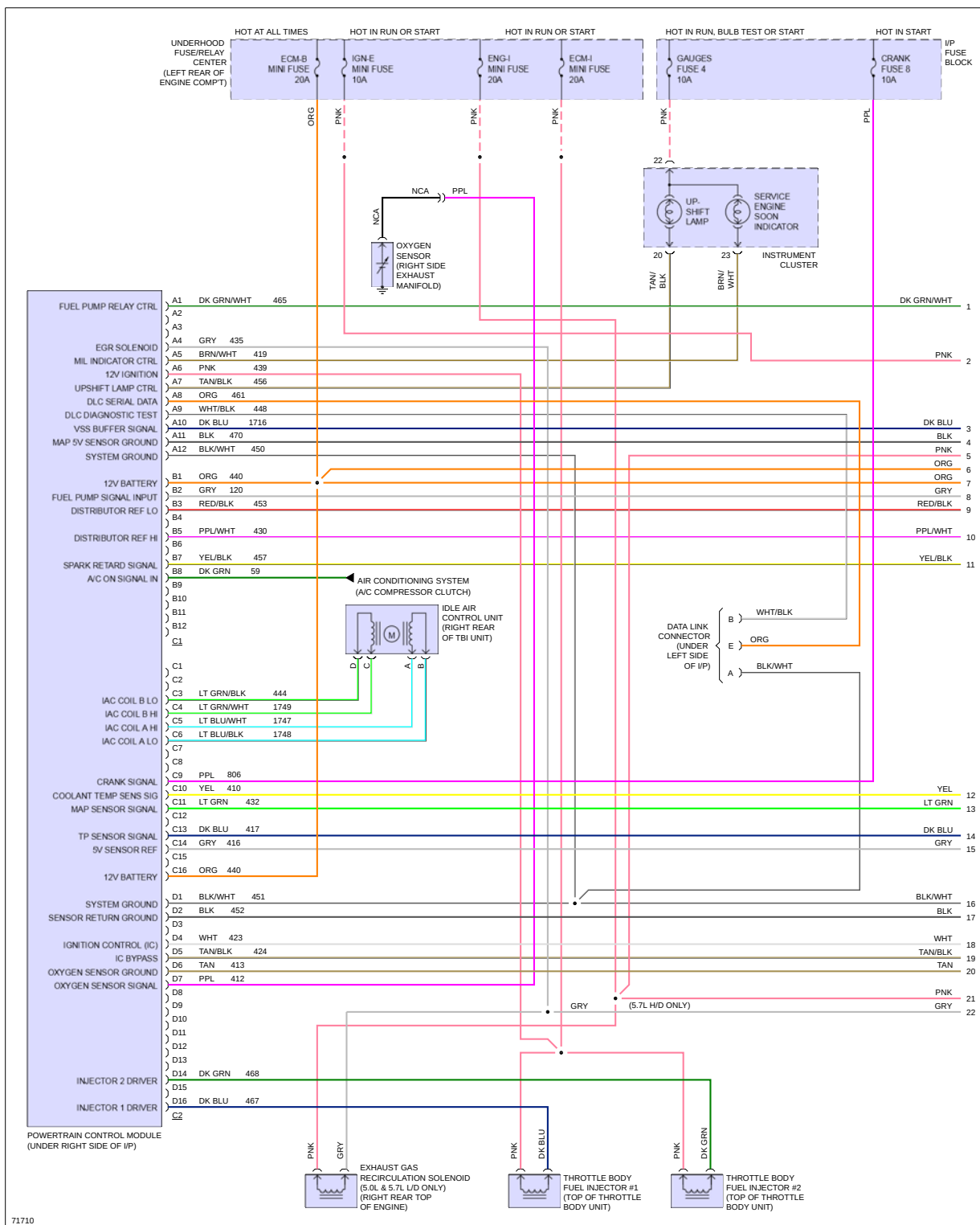
Fig 4: 5.7L (VIN K), Engine Performance Circuits, M/T (1 of 2)
