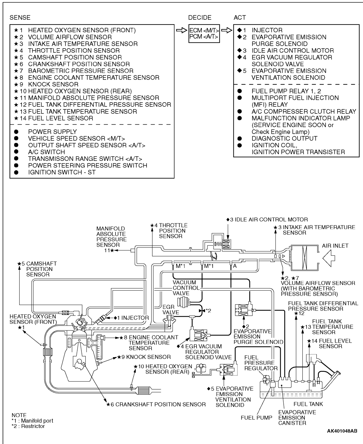
Fig 1: Multiport Fuel Injection (MFI) System Diagram
