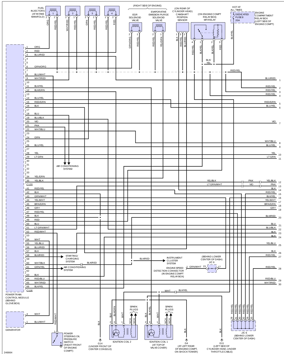
Fig 1: 2.0L, Engine Performance Circuit, A/T (1 of 3)
