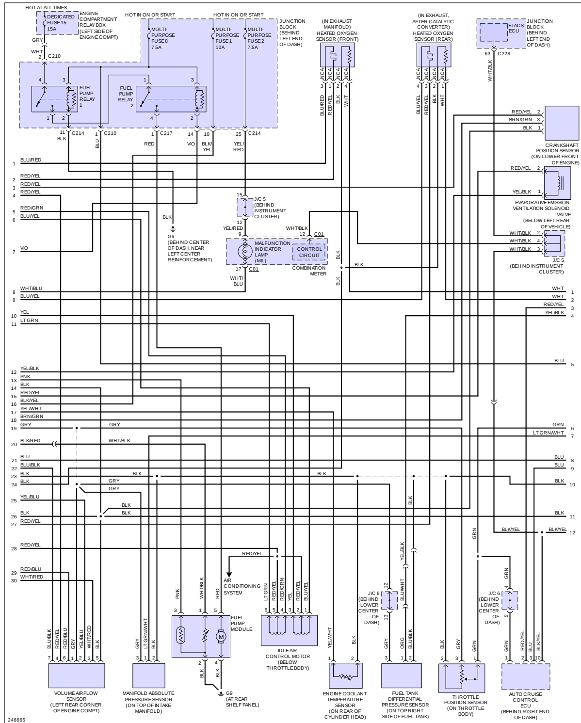
Fig 2: 2.0L, Engine Performance Circuit, A/T (2 of 3)
