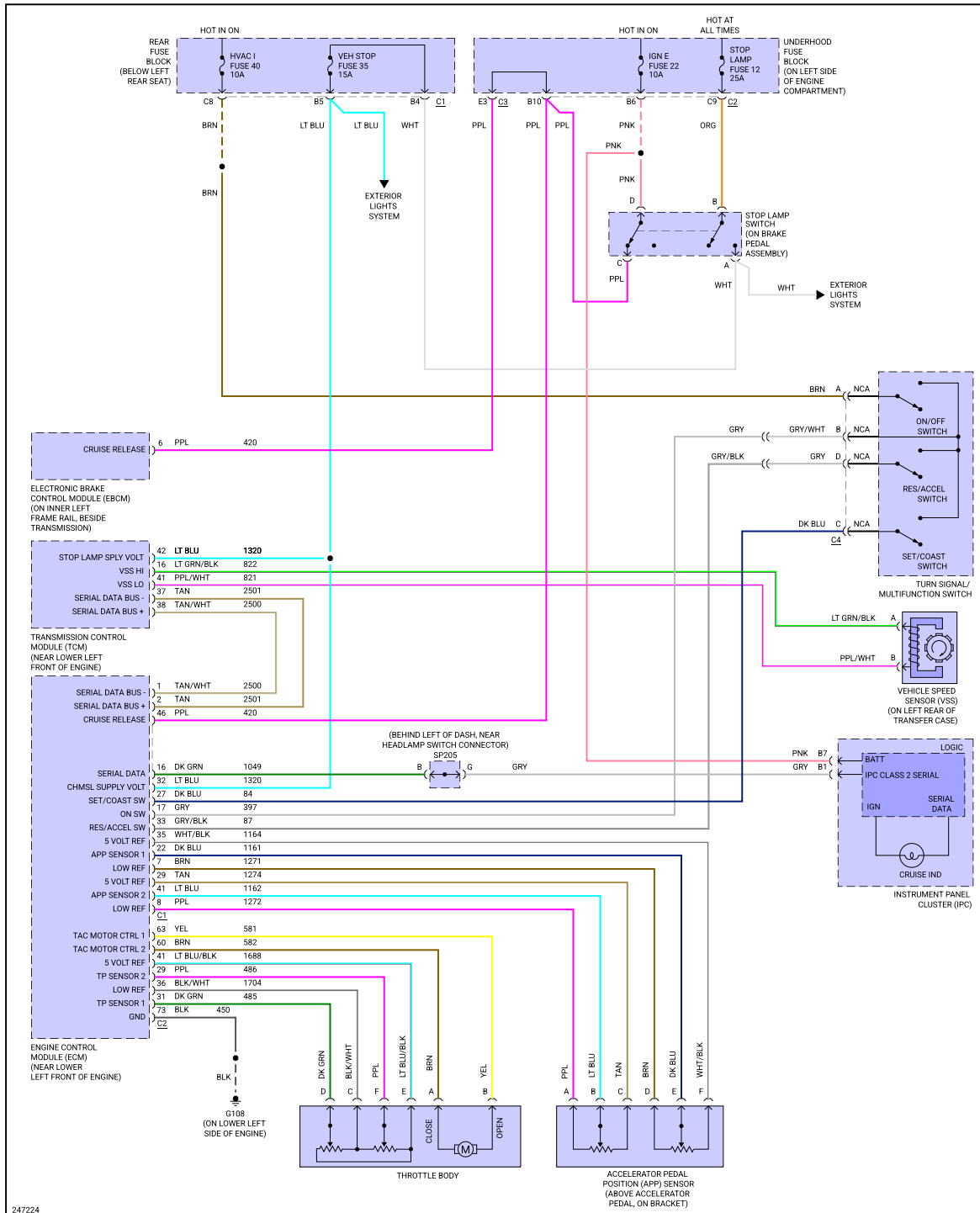
Fig 1: 5.3L, Cruise Control Circuit
