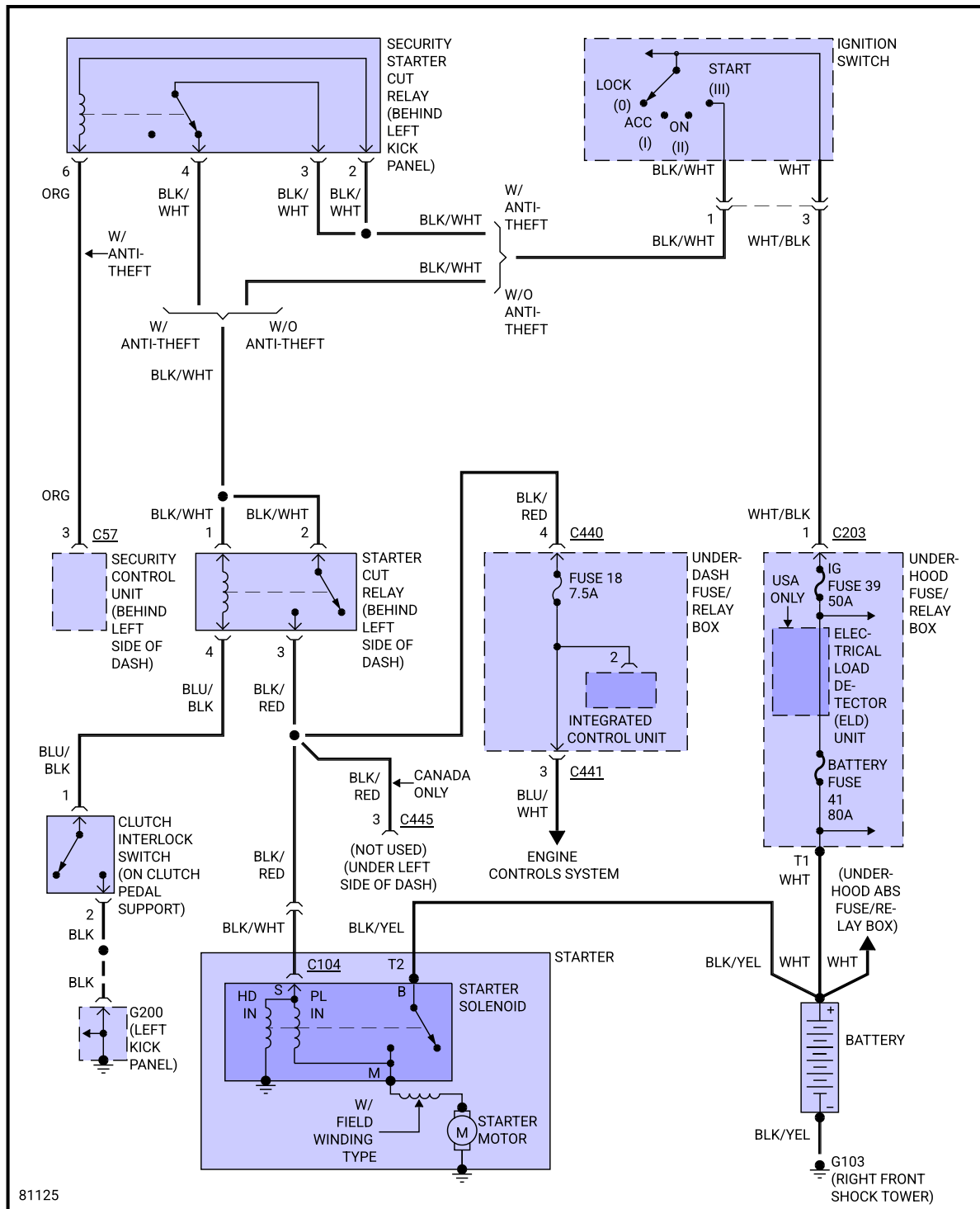
Fig 3: Starting Circuit, M/T
