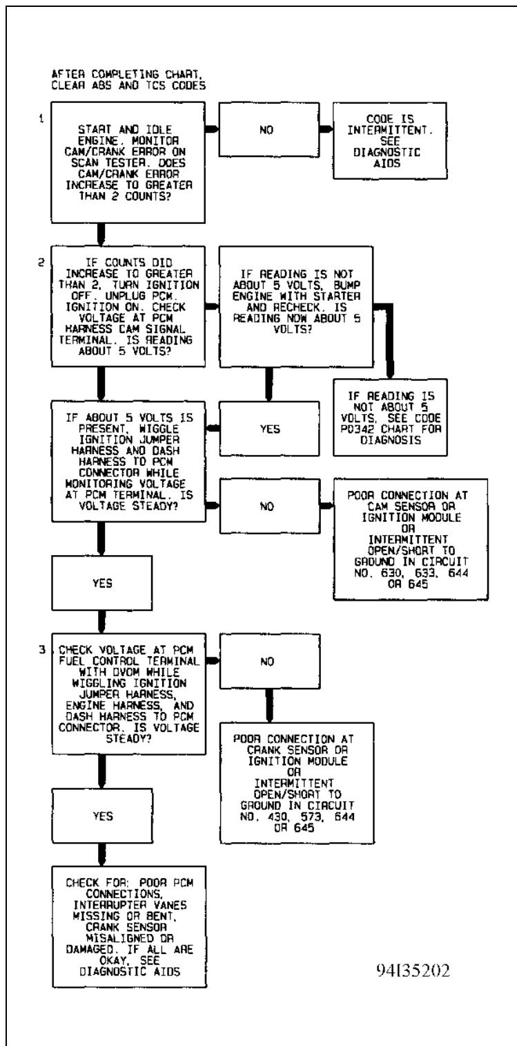
Fig 2: Code P0341 Flow Chart (3.8L) CAM/Crank Error
