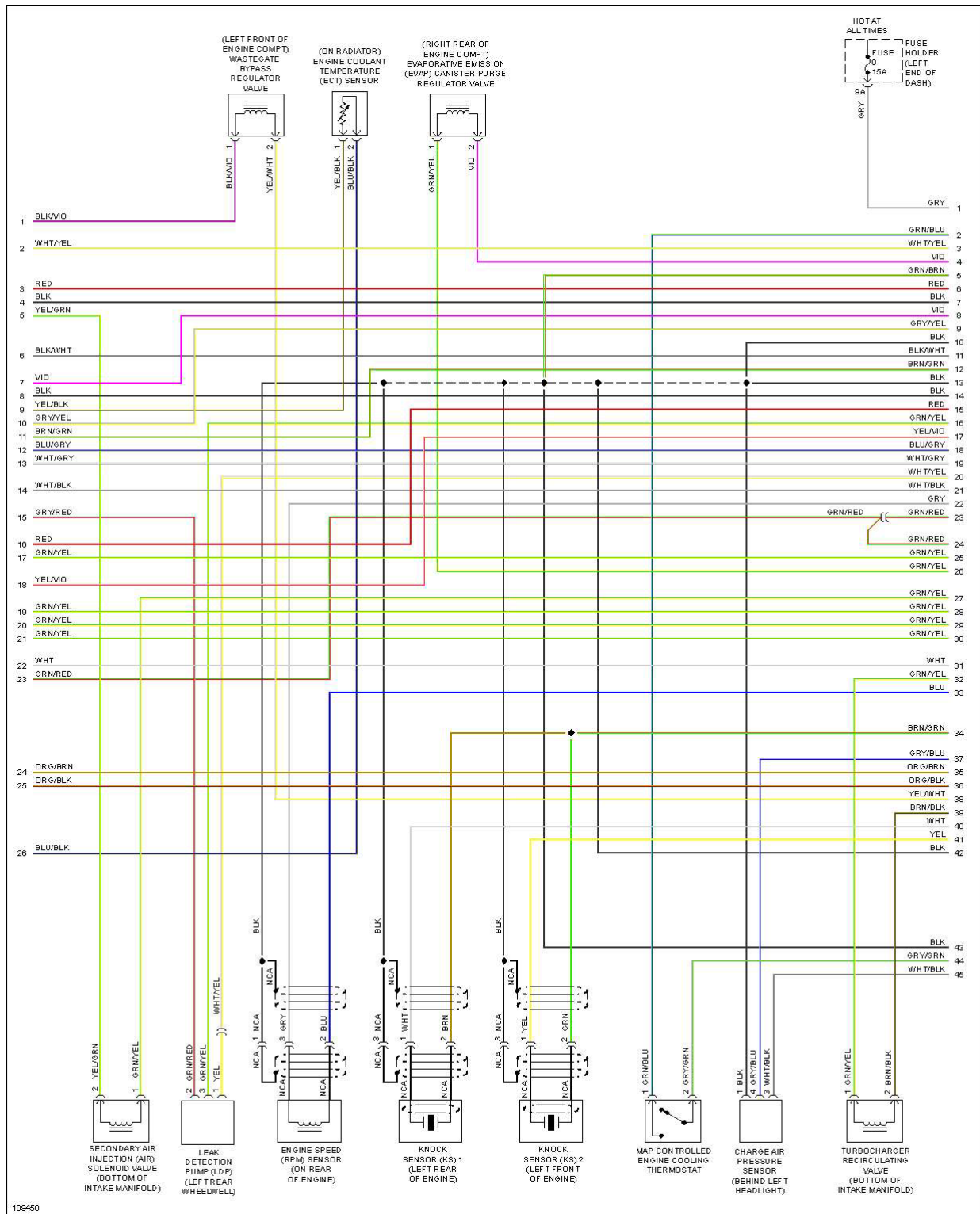
Fig. 17: 1.8L, Engine Performance Circuit (2 of 4)
