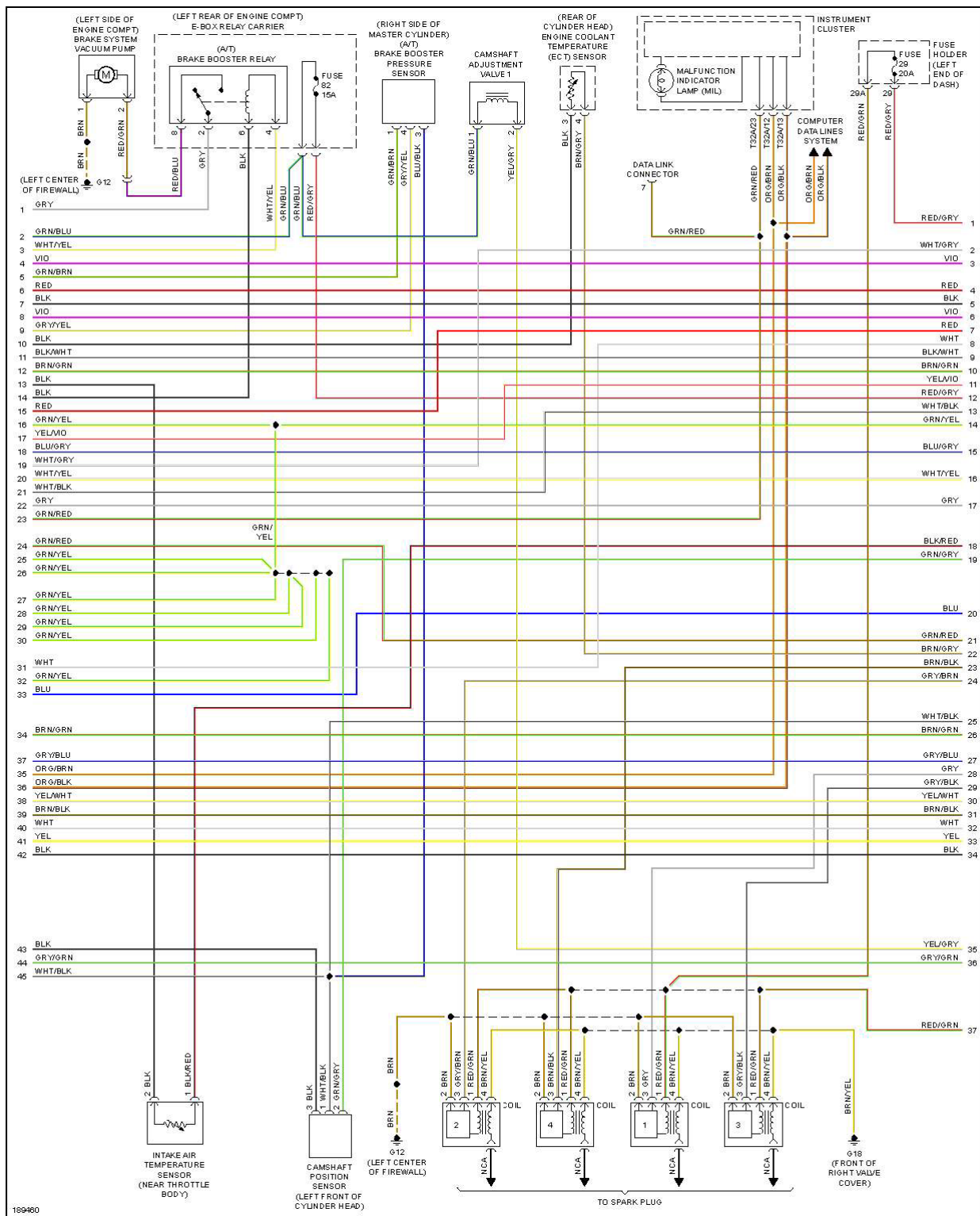
Fig. 18: 1.8L, Engine Performance Circuit (3 of 4)
