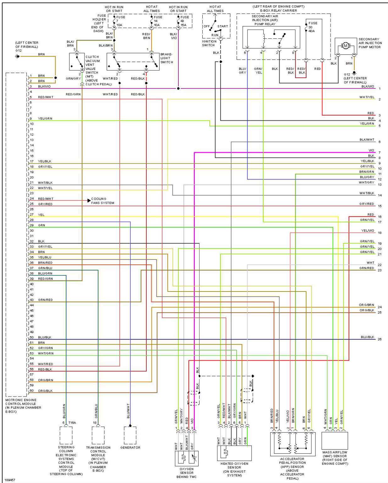
Fig. 16: 1.8L, Engine Performance Circuit (1 of 4)
