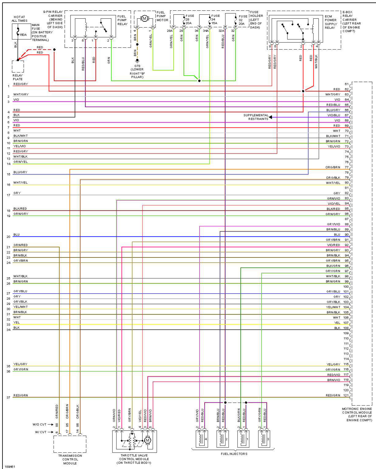
Fig. 19: 1.8L, Engine Performance Circuit (4 of 4)
