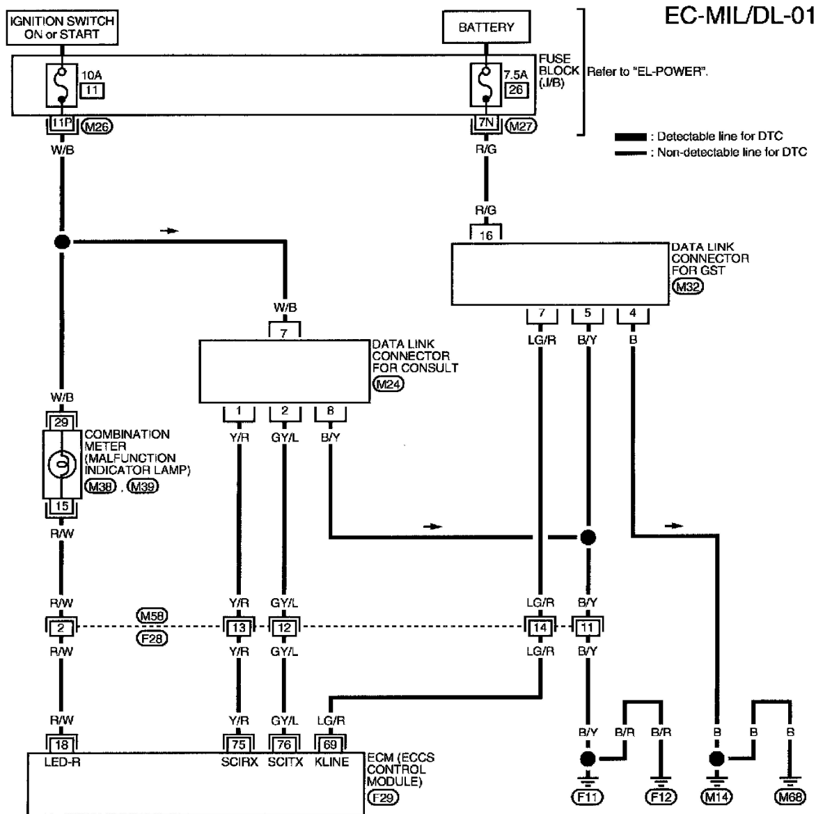
EC-MIL/DL-01 MIL &amp; Data Link Connectors
