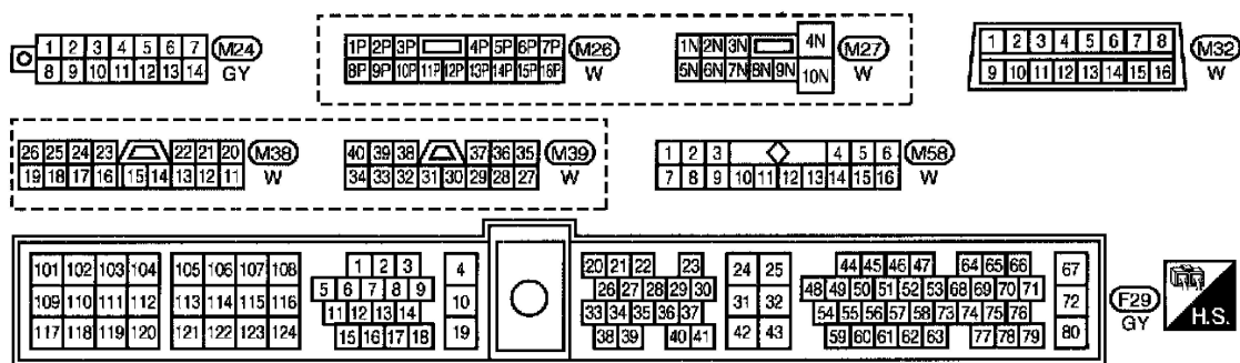
MIL &amp; Data Link Connectors
