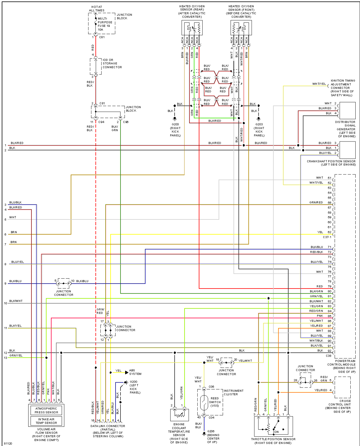
Fig. 12: 3.0L 12 Valve, Engine Performance Circuits (3 of 3)
