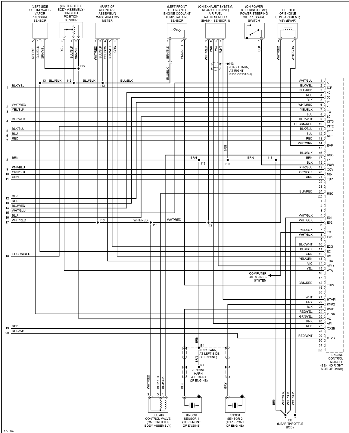
Fig. 24: 3.4L, Engine Performance Circuit, M/T W/ 2-Wheel Drive (3 of 3)
