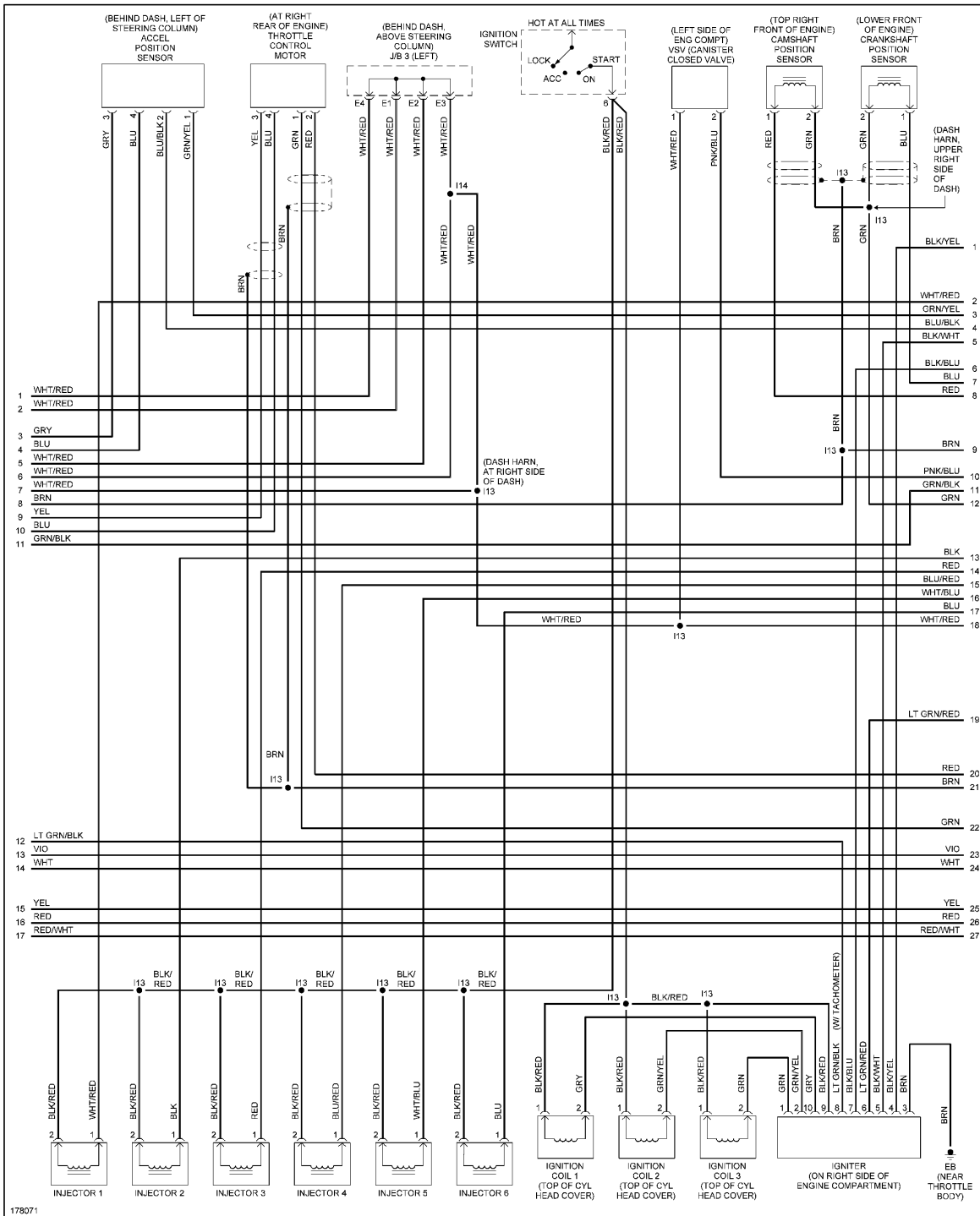
Fig. 20: 3.4L, Engine Performance Circuit, Except M/T W/ 2-Wheel Drive (3 of 4)
