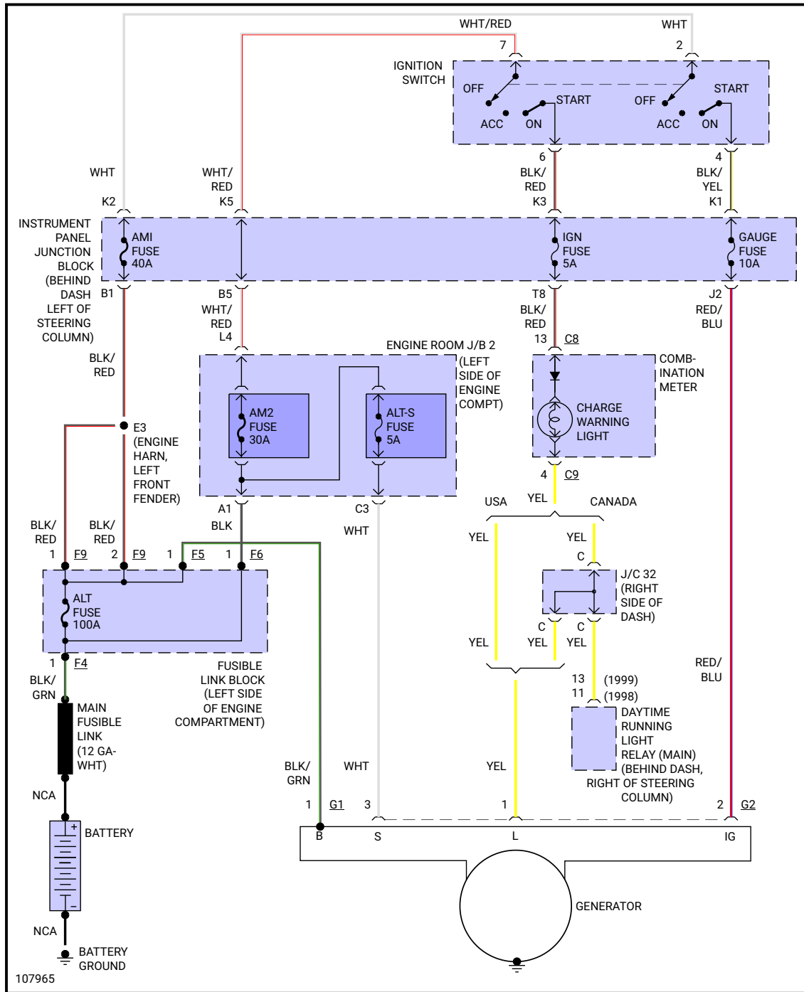
Fig 1: Charging Circuit
