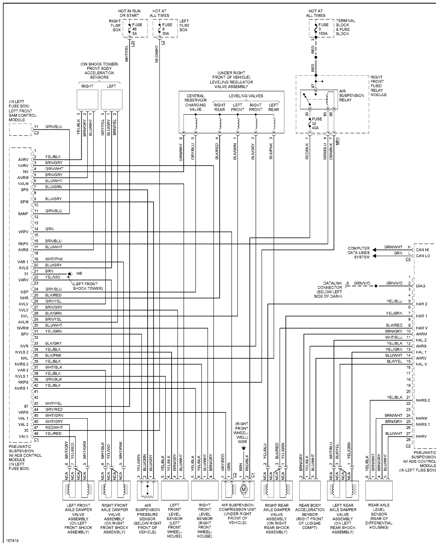
Fig. 16: Electronic Suspension Circuit
