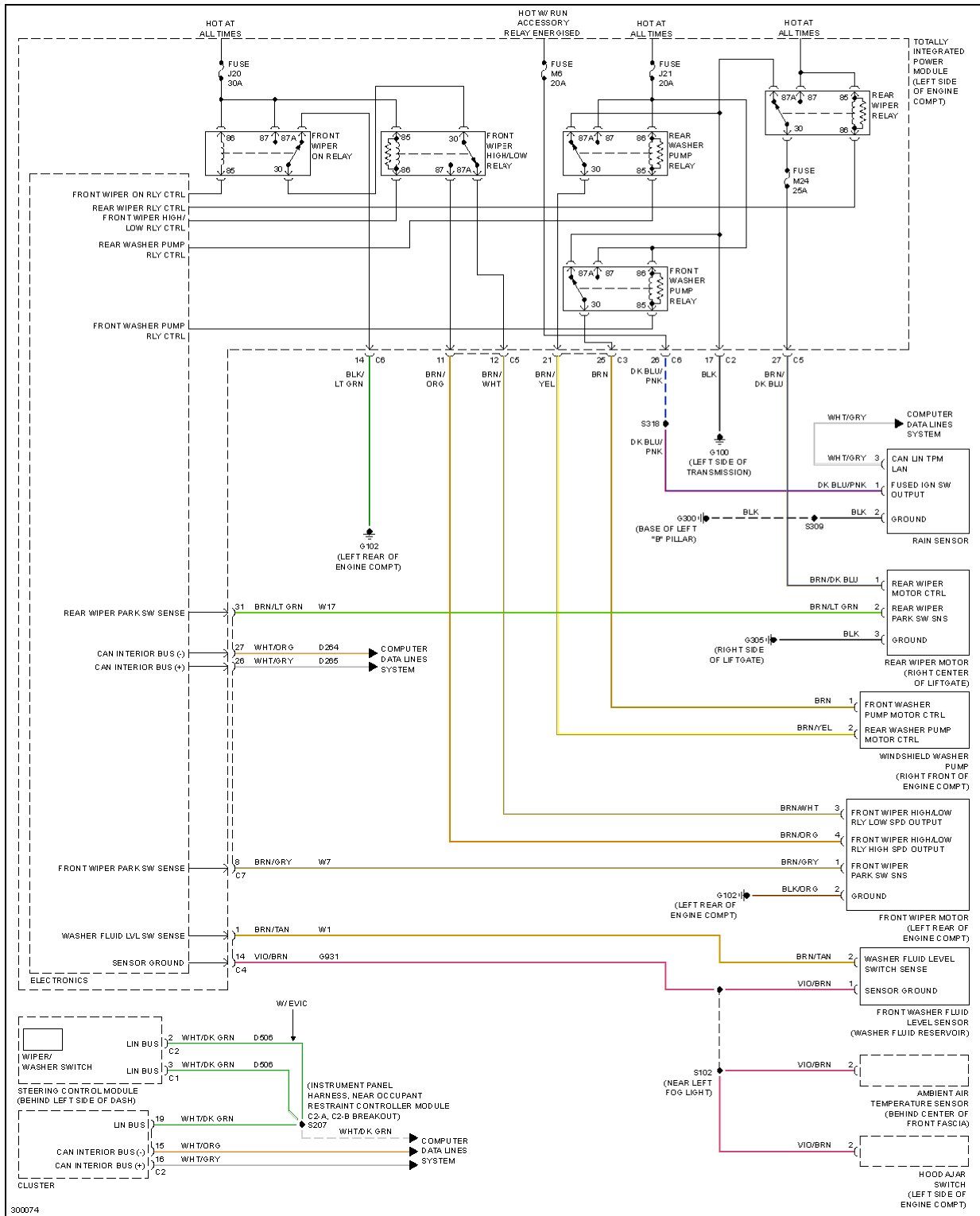
Fig. 94: Wiper/Washer Circuit
