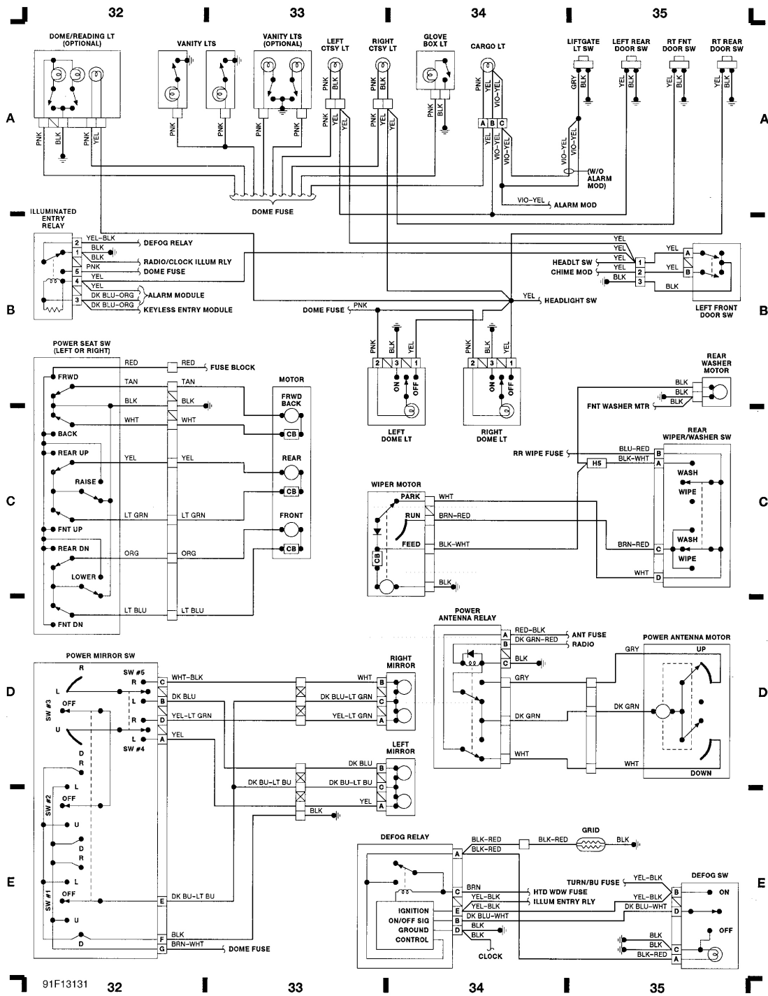
Fig. 9: Passenger Compartment (Grids 32-35)
