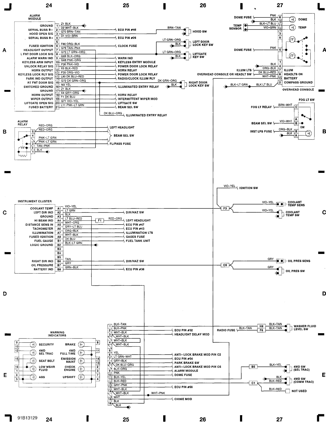
Fig. 7: Alarm Module, Instr Cluster, Warning Indicators (Grids 24-27)
