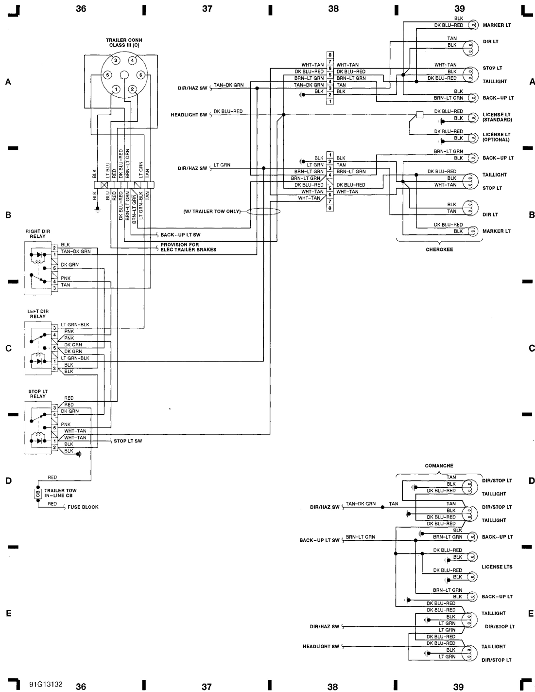
Fig. 10: Taillights (Grids 36-39)
