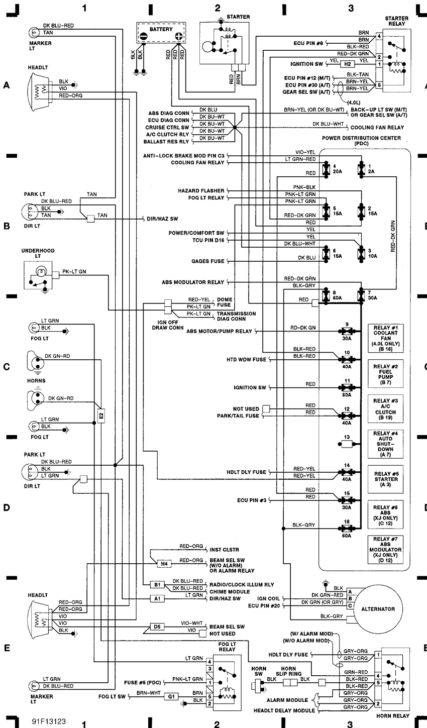
Fig. 1: Engine Compartment & Headlights (Grids 1-3)
