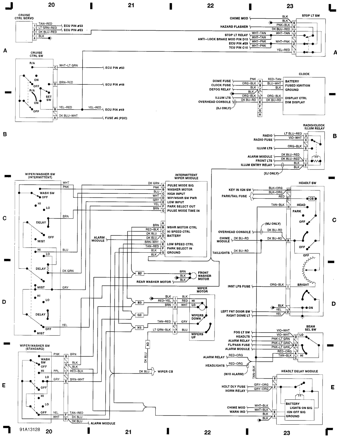
Fig. 6: Wiper/Washer, Wiper Module, Cruise Control Sw (Grids 20-23)
