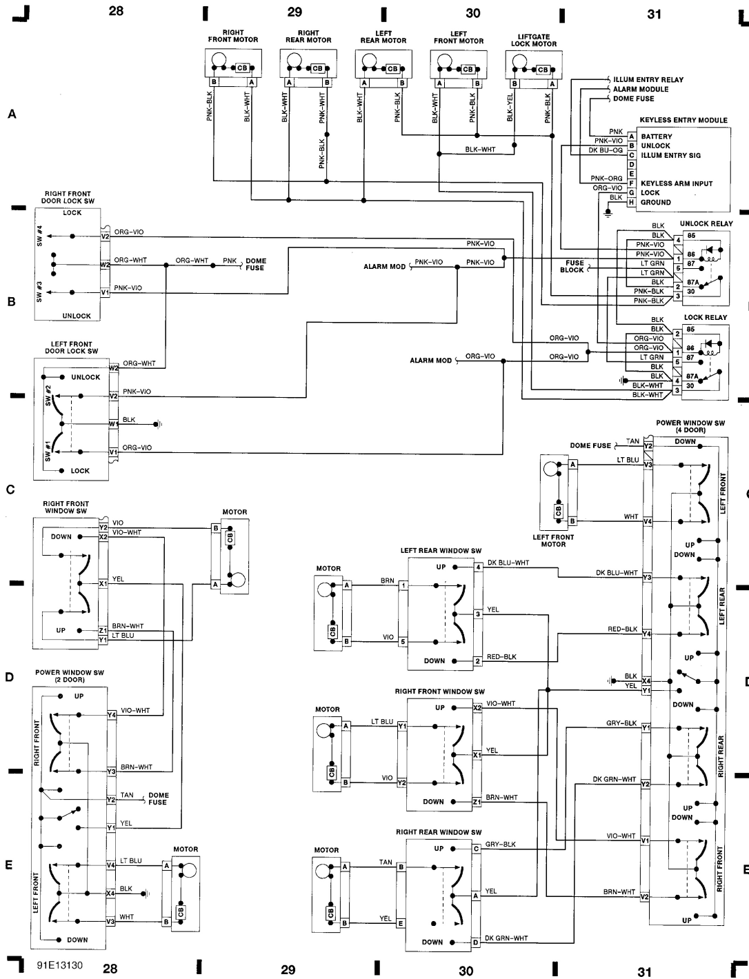
Fig. 8: Power Door & Window Modules (Grids 28-31)
