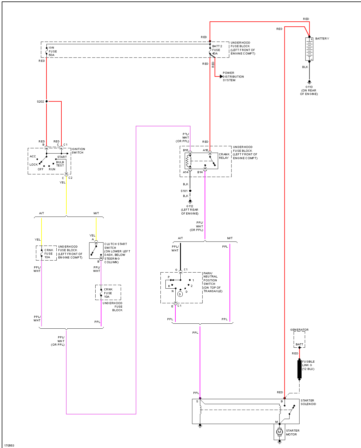
Fig. 40: Starting Circuit
