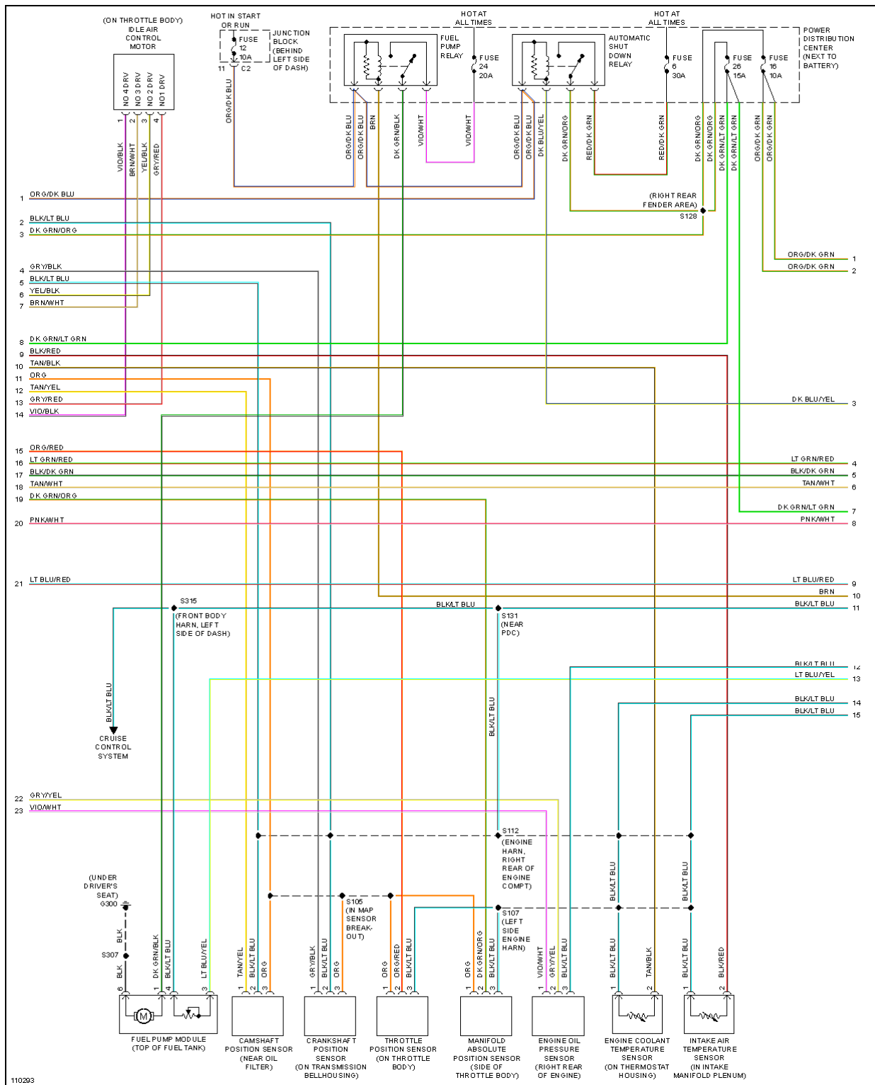
Fig. 11: 4.0L, Engine Performance Circuits (2 of 3)
