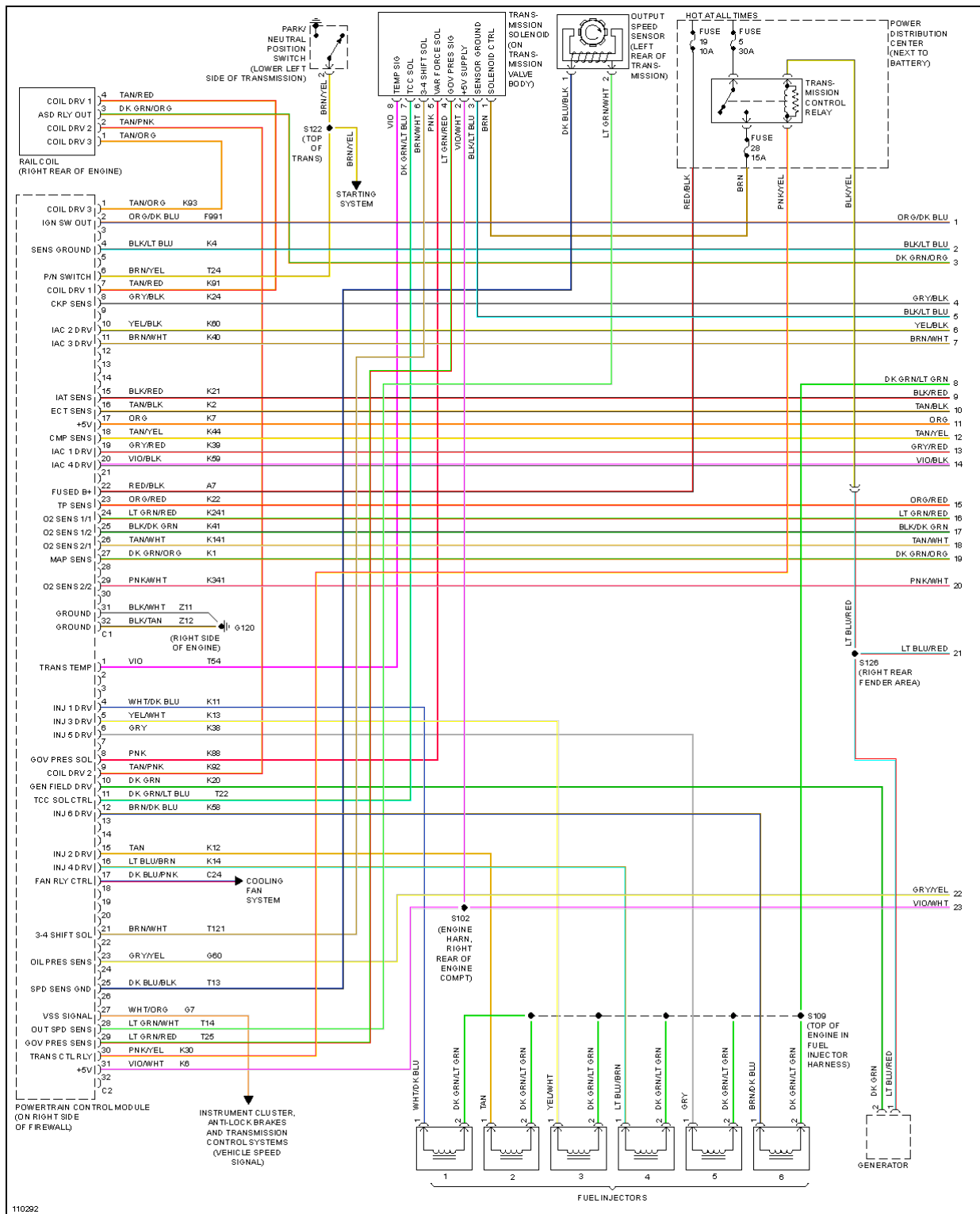
Fig. 10: 4.0L, Engine Performance Circuits (1 of 3)
