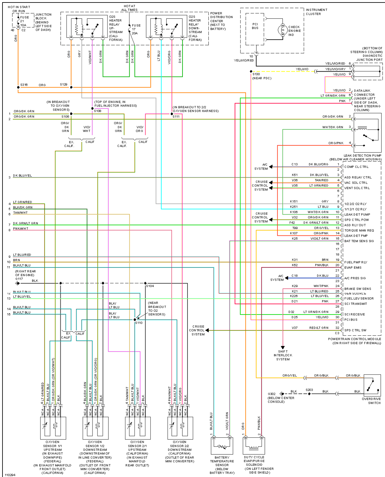
Fig. 12: 4.0L, Engine Performance Circuits (3 of 3)
