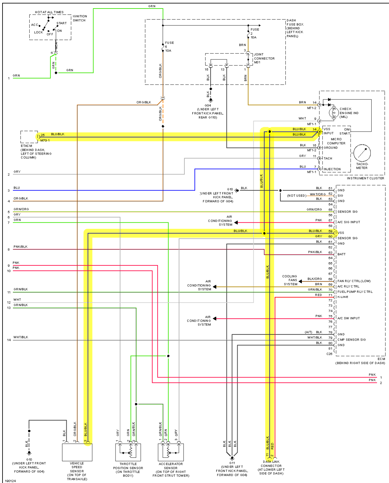
Fig. 12: 1.6L, Engine Performance Circuit (3 of 4)
