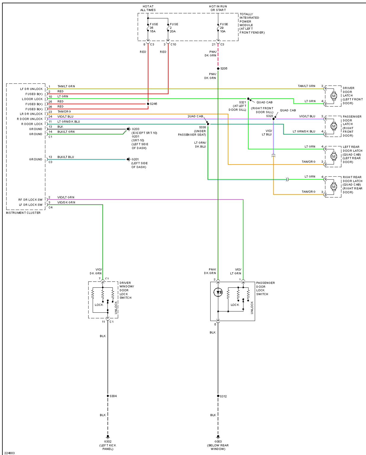
Fig. 55: Power Door Locks Circuit
