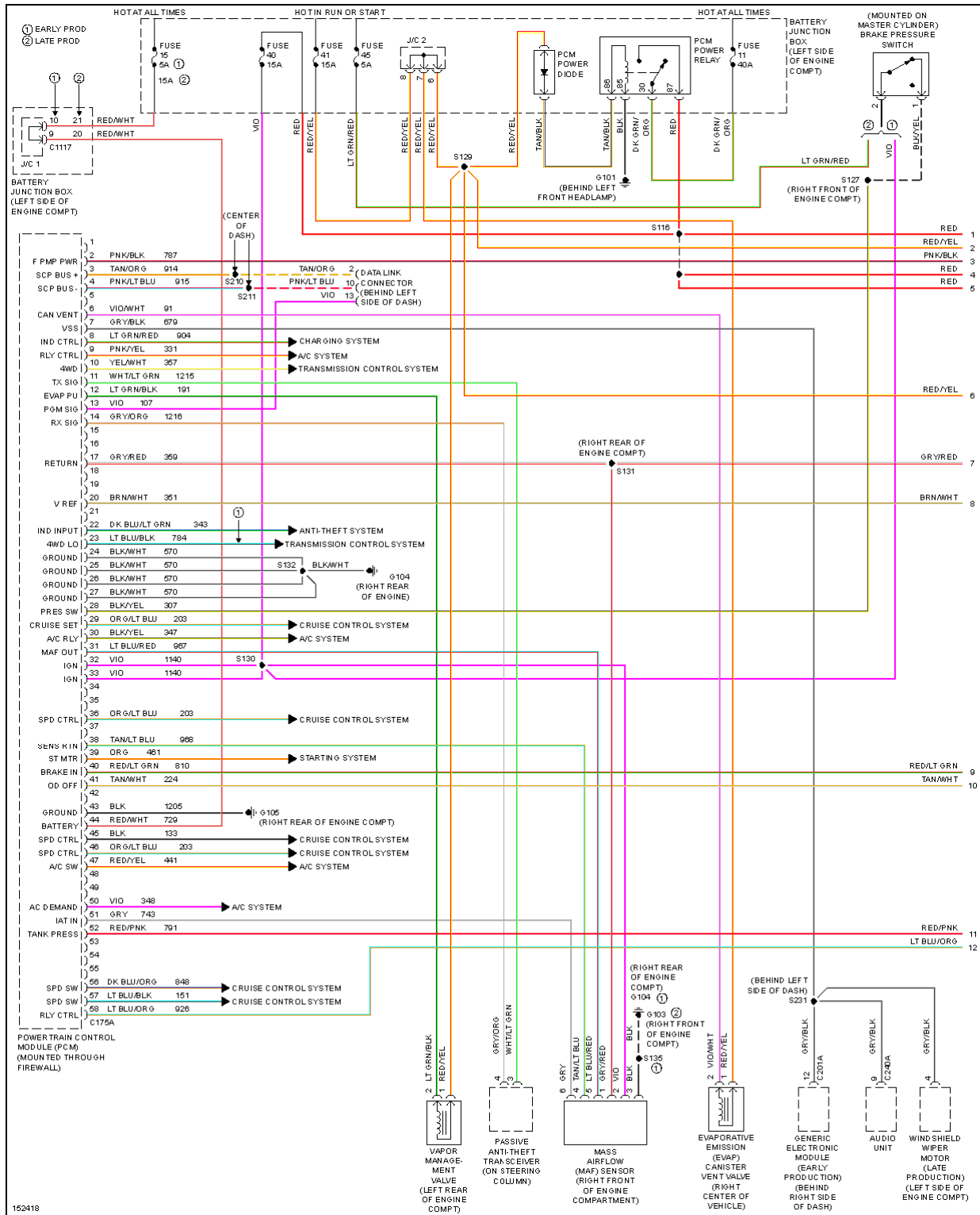
Fig. 23: 4.0L, Engine Performance Circuits (1 of 4)
