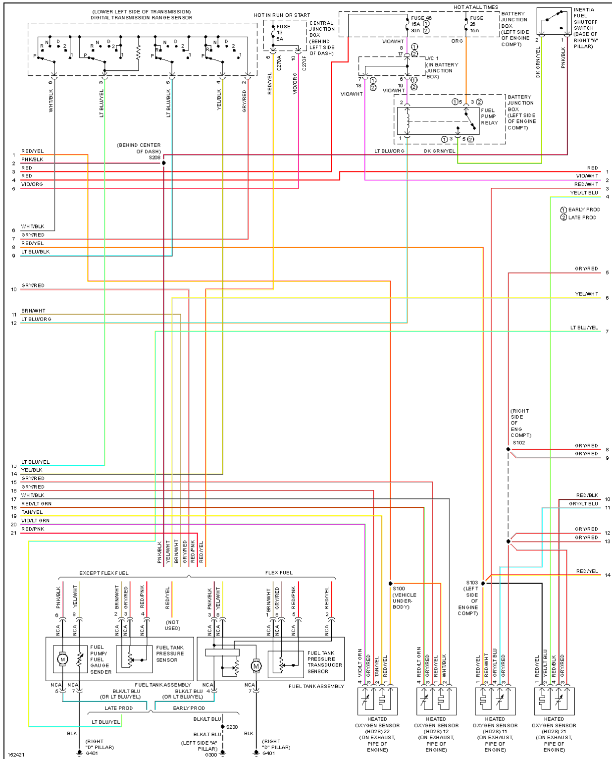
Fig. 25: 4.0L, Engine Performance Circuits (3 of 4)
