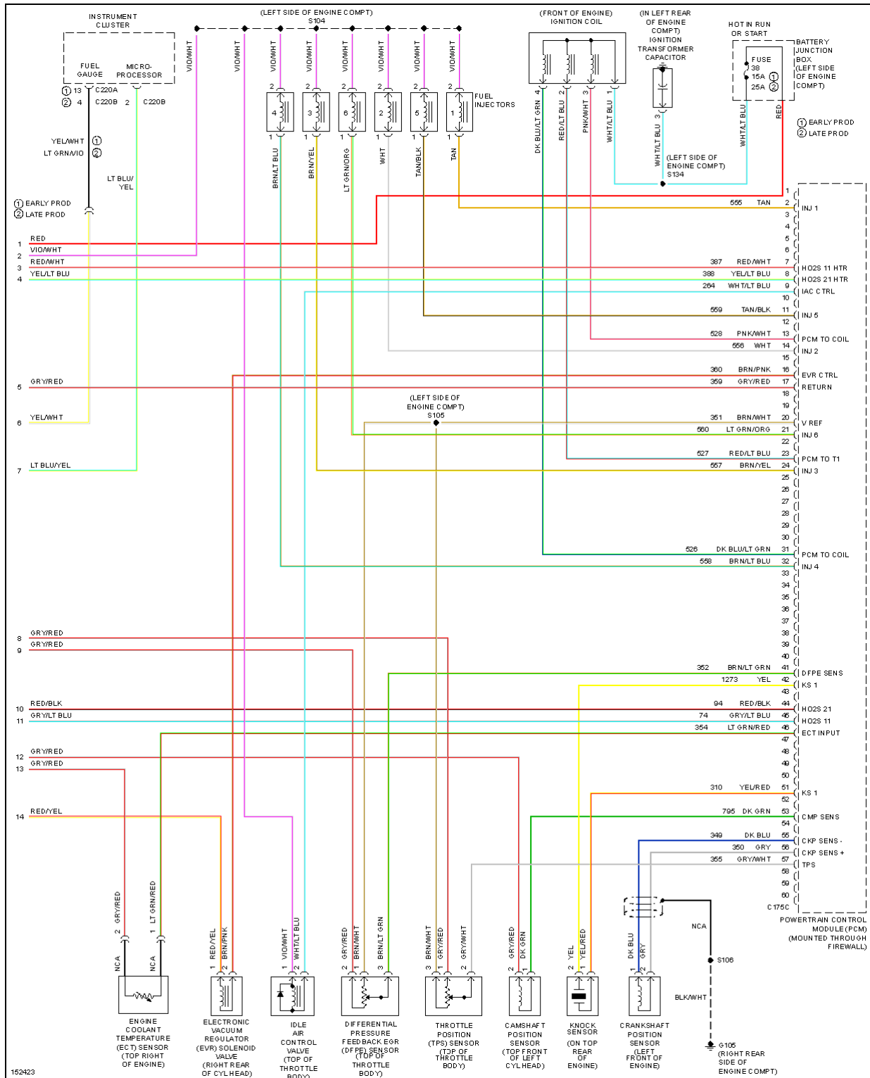
Fig. 26: 4.0L, Engine Performance Circuits (4 of 4)
