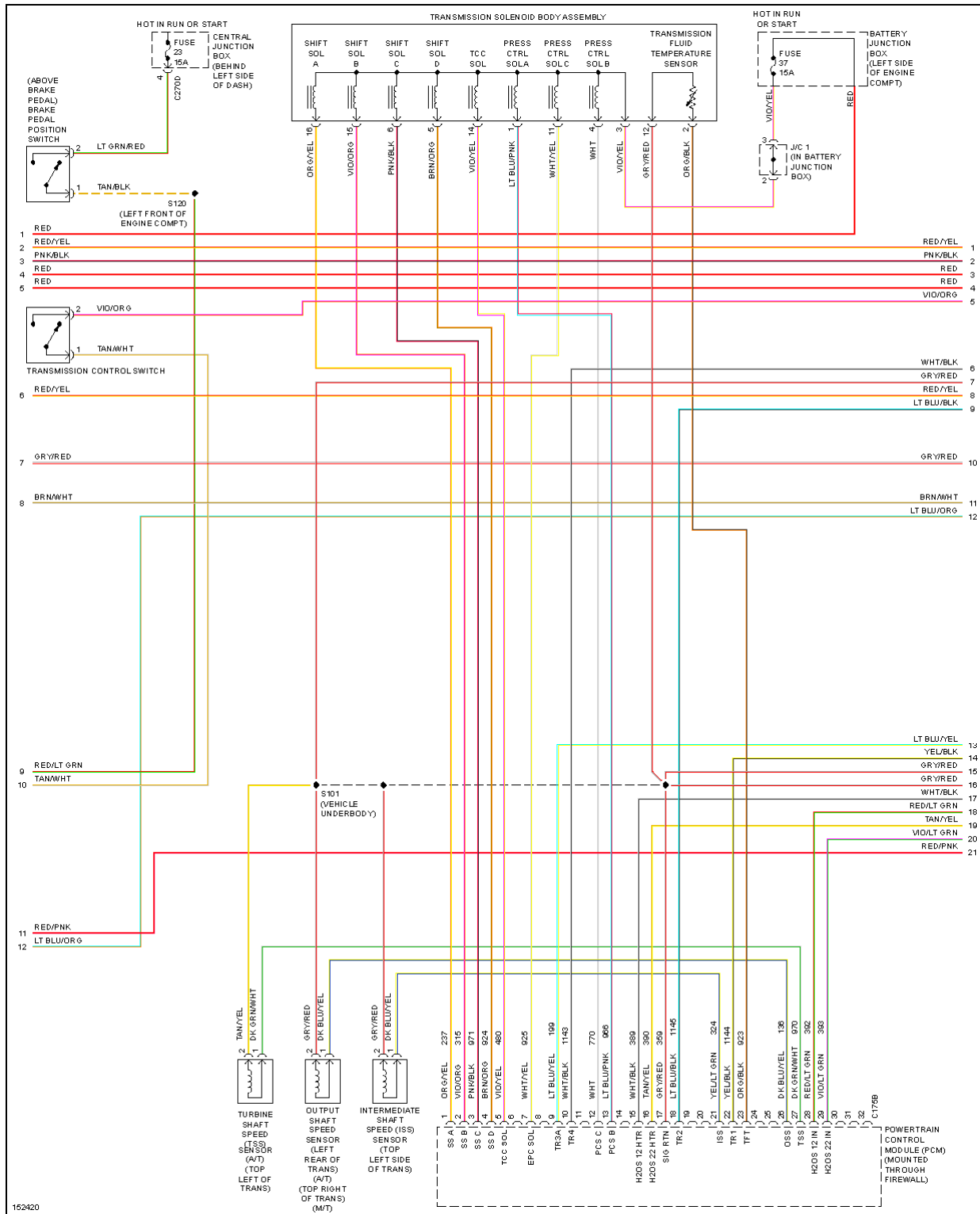
Fig. 24: 4.0L, Engine Performance Circuits (2 of 4)
