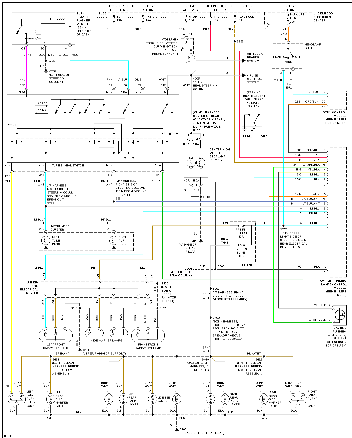
Fig. 16: Exterior Lamps Circuit
