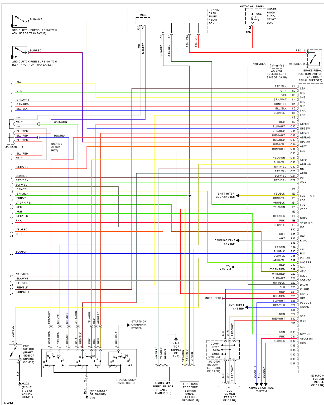
Fig. 27: 2.4L, Engine Performance Circuit (4 of 4)
