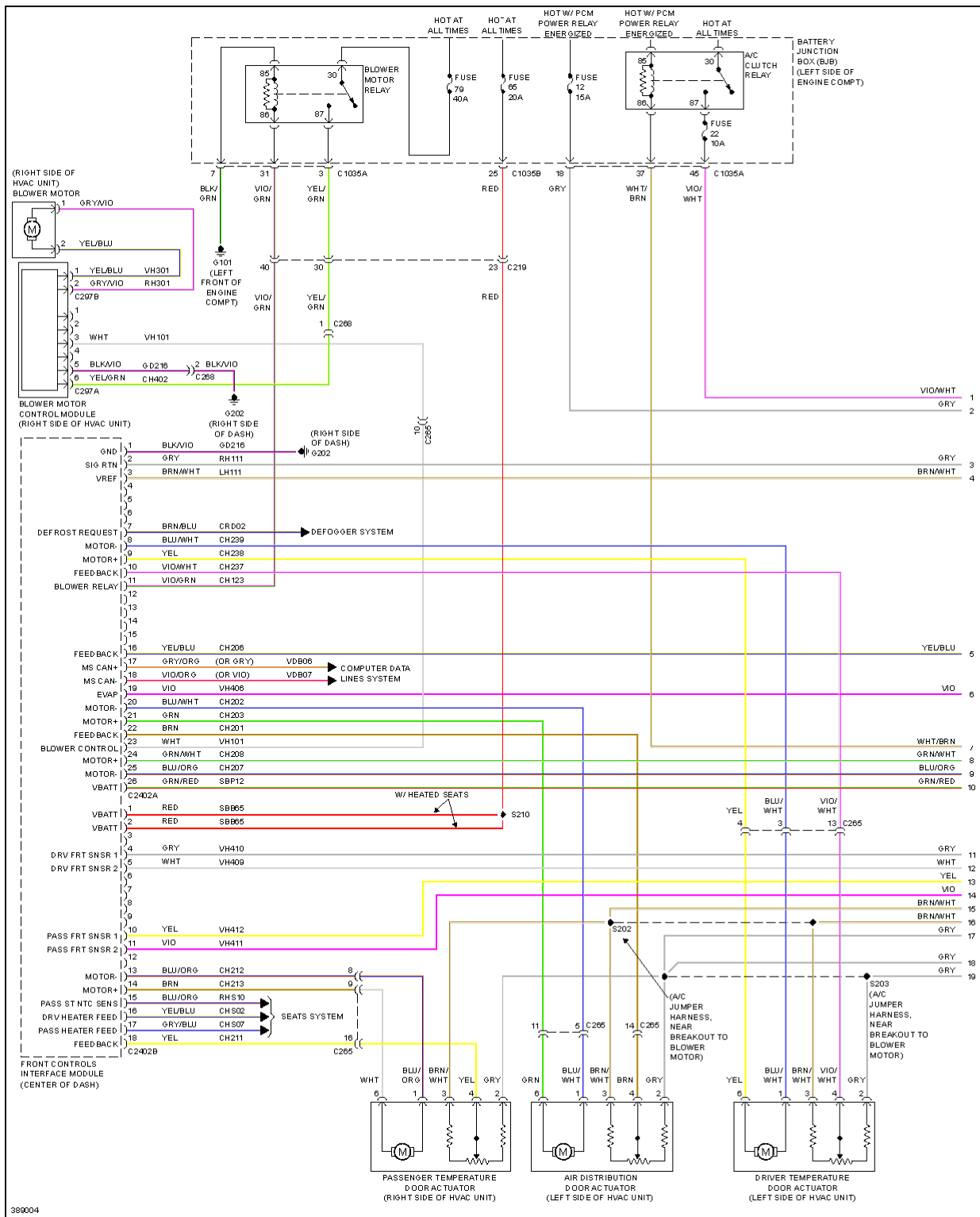
Fig. 1: Automatic A/C Circuit, Except Hybrid (1 of 3)
