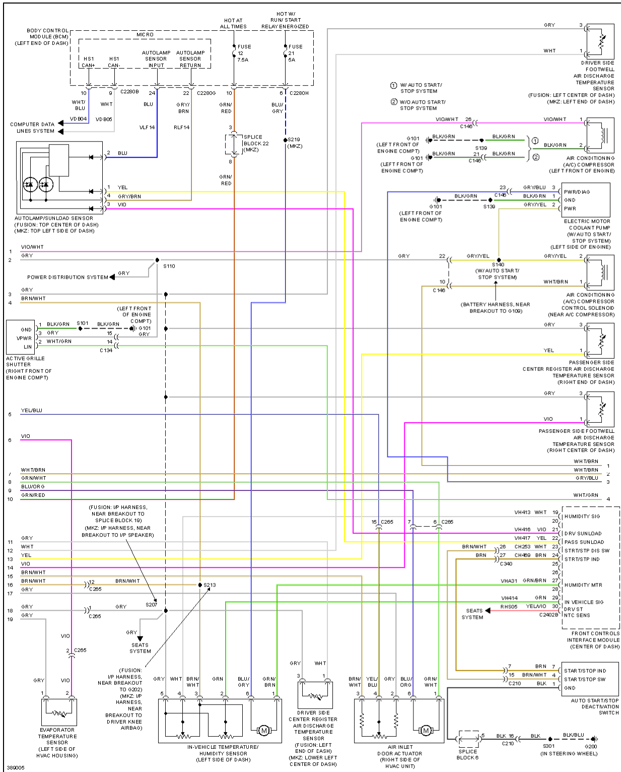
Fig. 2: Automatic A/C Circuit, Except Hybrid (2 of 3)
