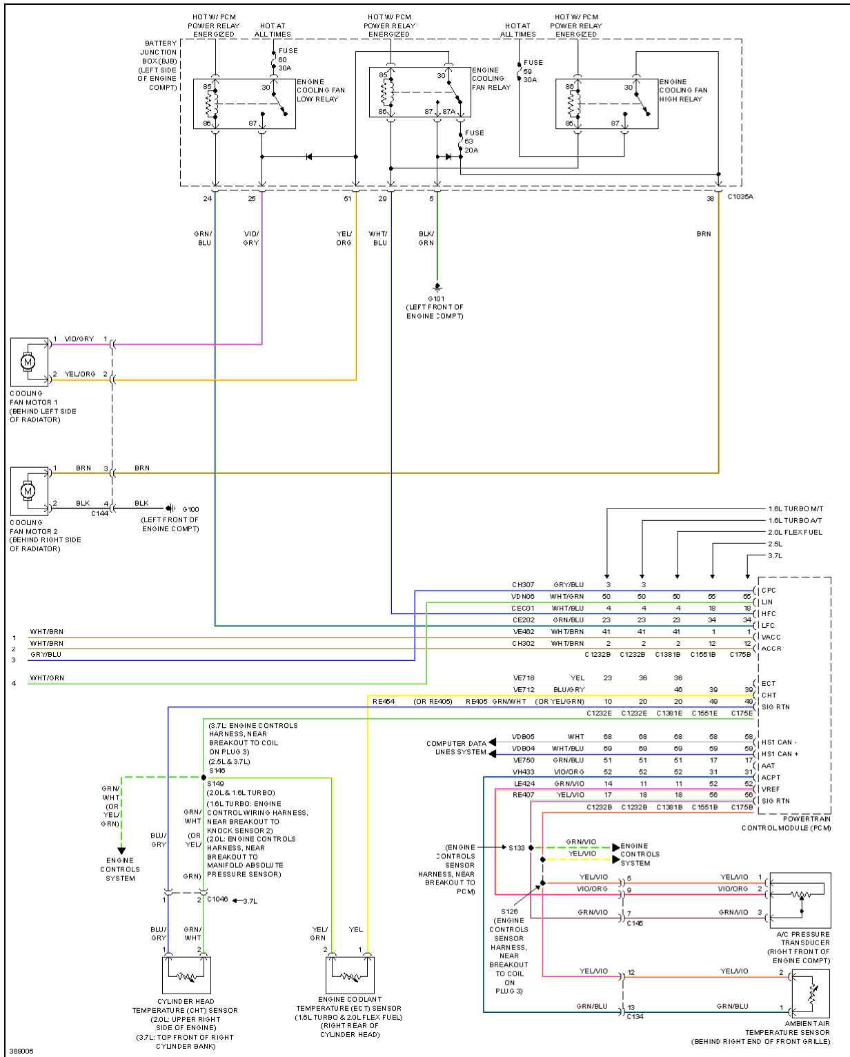
Fig. 3: Automatic A/C Circuit, Except Hybrid (3 of 3)
