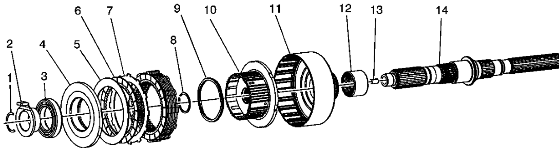
Fig. 18: Clutch Components
