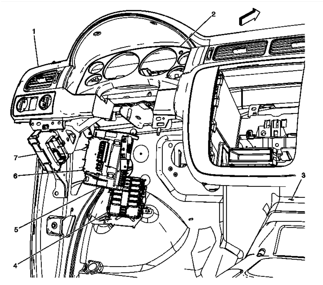
Fig. 6: Below the I/P Courtesy of GENERAL MOTORS CORP.
