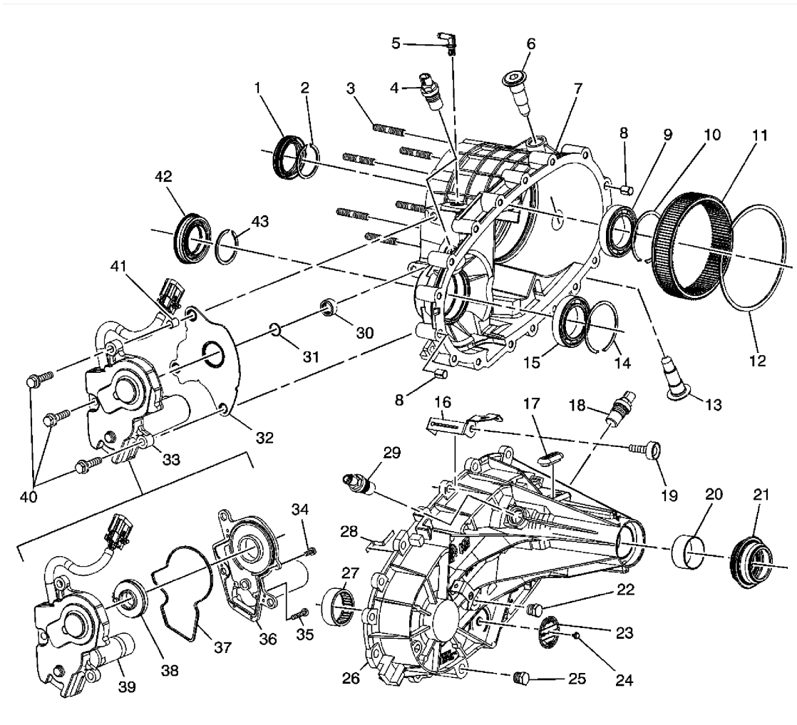
Fig. 16: Case Half Components Disassembled View Courtesy of GENERAL MOTORS CORP.
